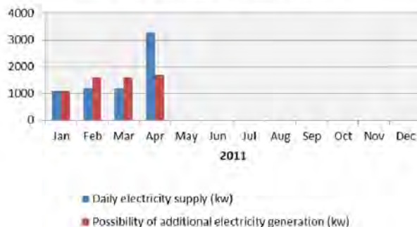
Electricity (kw) supplied by EDTL Covalima
