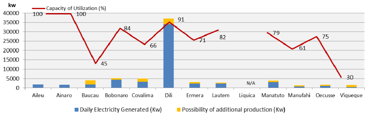
Comparison of Generation of Electricity by EDTL 15 April 2011
