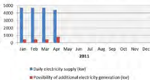
Electricity (kw) supplied by EDTL Bobonaro
